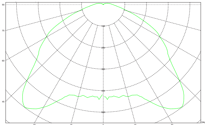
Illuminance angle
