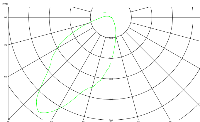
Illuminance angle, long side to ceiling
